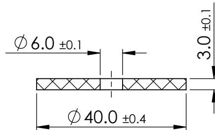
SECTION X-X
